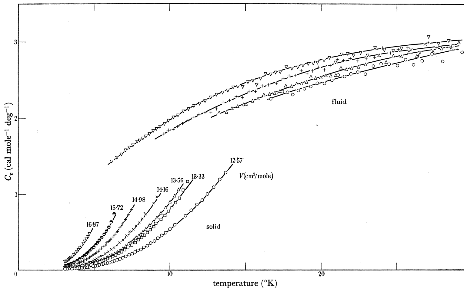
FIGURE 6. The specific heat at constant volume of solid and fluid 3 He at various volumes.
