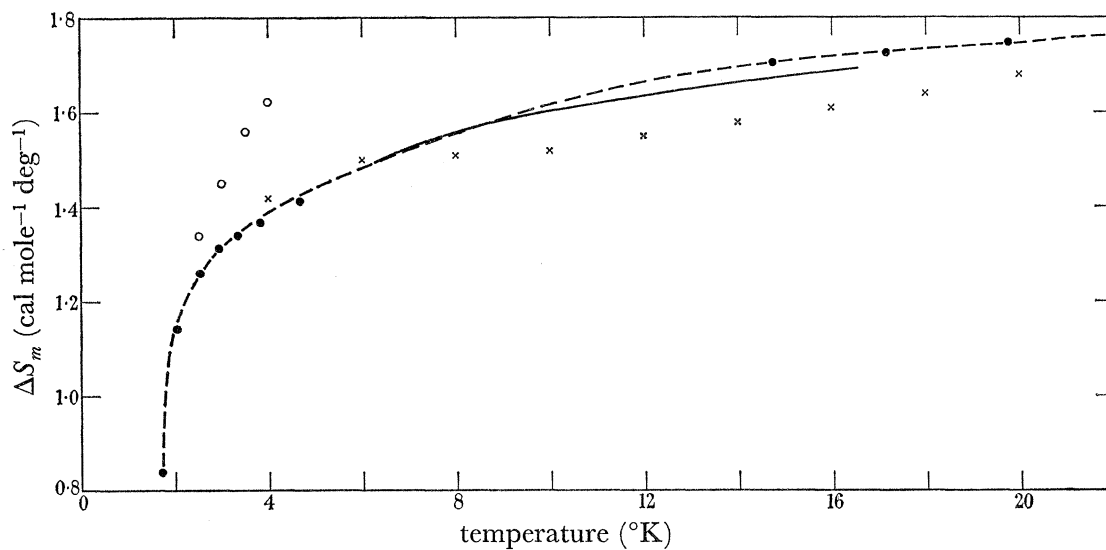
FIGURE 11. The melting entropy of ^4\text{He} as a function of temperature. —, This work; --●--●, Grilly & Mills (1959); \times , Dugdale & Simon (1953); \circ , Keesom & Keesom (1936).
