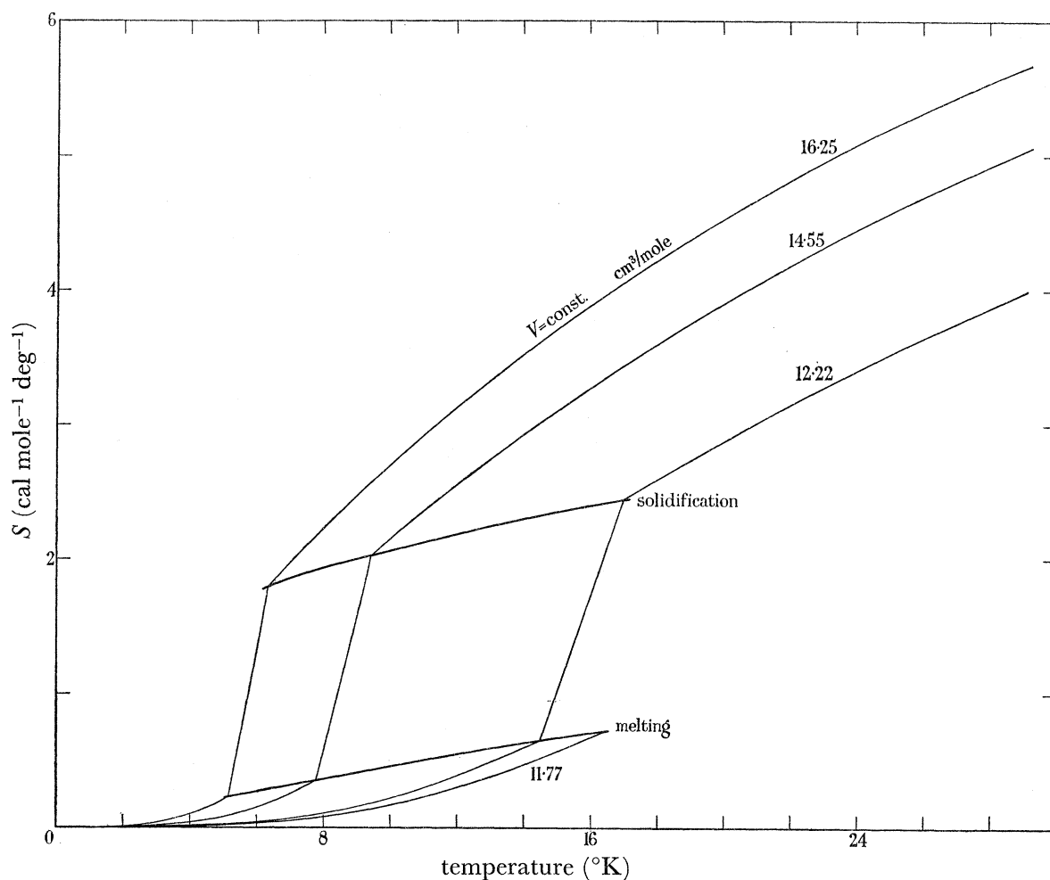
FIGURE 9. The entropy of 4 He. The numbered lines are lines of constant volume.
