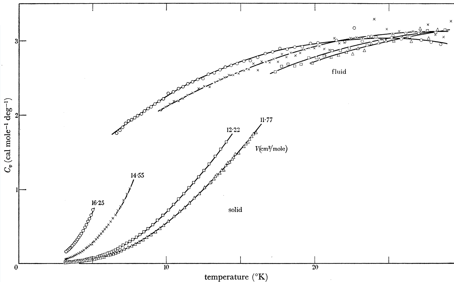
FIGURE 5. The specific heat at constant volume of solid and fluid 4 He at various volumes.
