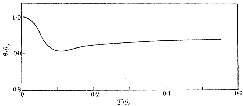
FIGURE 14. The dependence of \theta_D on temperature as calculated for an f.c.c. lattice (after Leighton 1948). The precise form of the curve depends on the force constants chosen.
