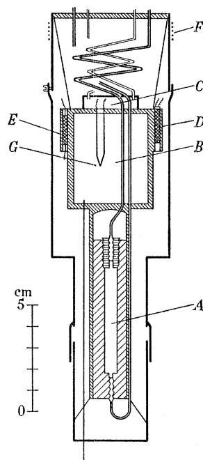
FIGURE 2. Calorimeter assembly and adiabatic shield.
