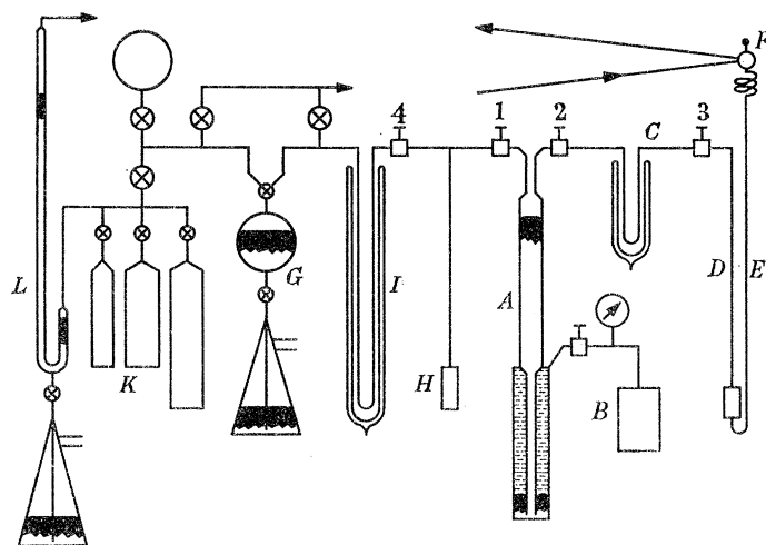
FIGURE 4. Schematic diagram of the gas handling assembly.
